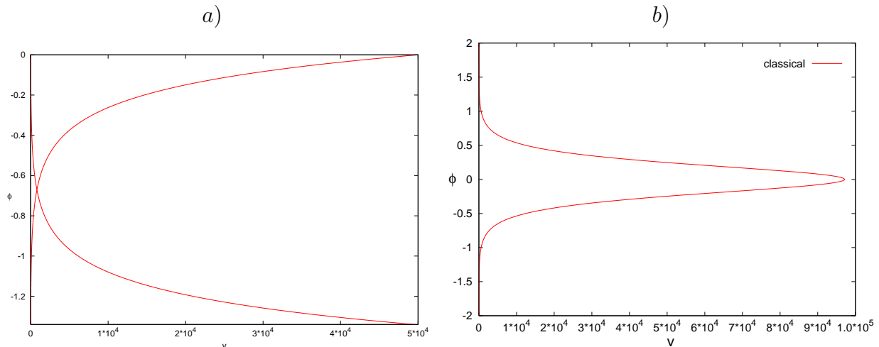
FIG. 1: Dynamics of FLRW universes with zero cosmological constant and a massless scalar field. Classical trajectories are plotted in the v - \phi plane, where v denotes the volume and \phi the scalar field. a) k=0 trajectories. b) A k=1 trajectory.
