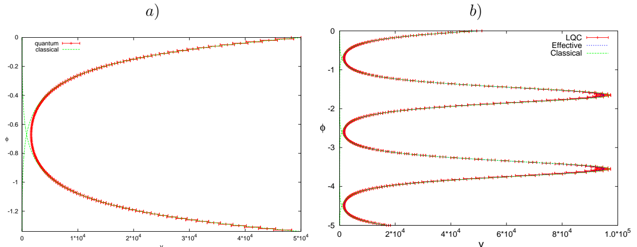
FIG. 2: In the LQC evolution of models under consideration, the big bang and big crunch singularities are replaced by quantum bounces. Expectation values and dispersion of the volume operator \hat{V}_\phi , are compared with the classical trajectory and the trajectory from effective Friedmann dynamics. The classical trajectory deviates significantly from the quantum evolution at the Planck scale and evolves into singularities. The effective trajectory provides an excellent approximation to quantum evolution at all scales. a) The k=0 case. In the backward evolution, the quantum evolution follows our post big-bang branch at low densities and curvatures but undergoes a quantum bounce at matter density \rho \sim 0.41\rho_{\text{PL}} and joins on to the classical trajectory that was contracting to the future. b) The k=1 case. The quantum bounce occurs again at \rho \sim 0.41\rho_{\text{PL}} . Since the big bang and the big crunch singularities are resolved the evolution undergoes cycles. In this simulation p_{(\phi)}^* = 5 \times 10^3 , \Delta p_{(\phi)}/p_{(\phi)}^* = 0.018 , and v^* = 5 \times 10^4 .
